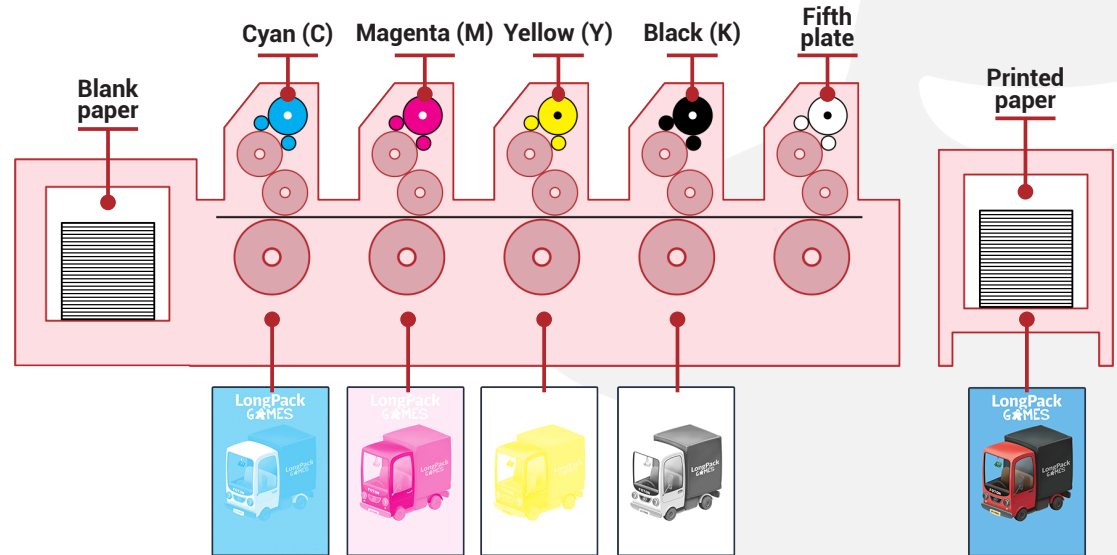
An offset printing press with 4+1 colors
